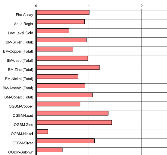
Mean of Absolute Standardized Values Standard Deviations
