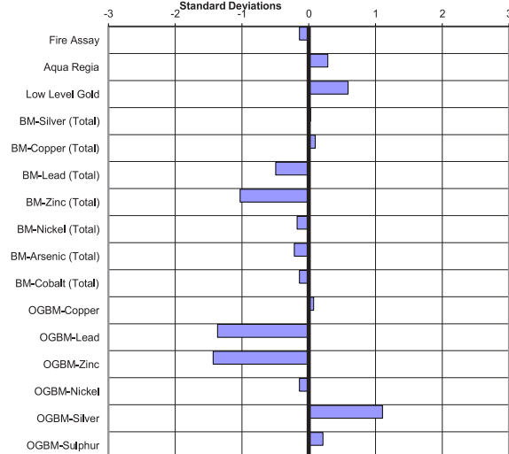
Mean of Standardized Values Standard Deviations
